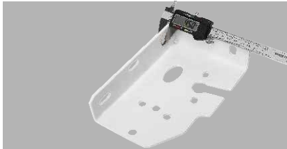
Normal curved arm side plate
